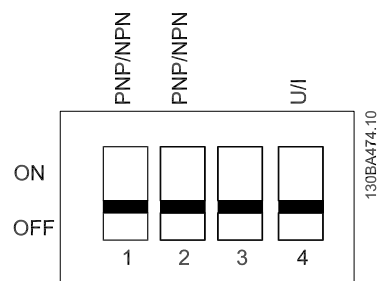
3.9: S200 Switches 1-4.
