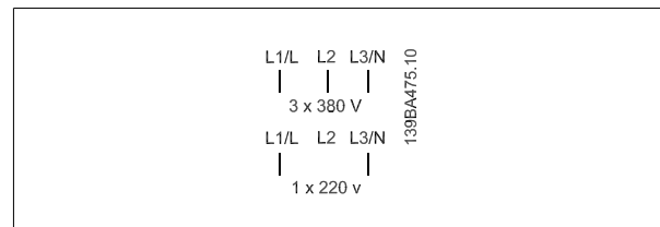
3.2: Three-phase and single-phase wire connections.
