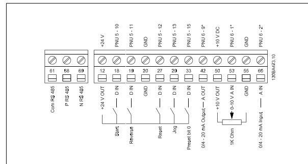
3.7: Overview of control terminals in the PNP configuration and factory settings.
