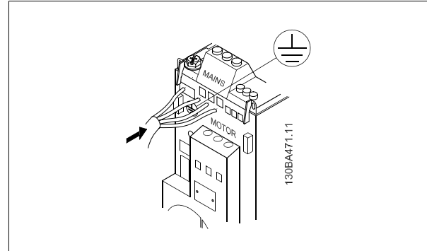
3.1: Mounting of ground cable and line power wires.
