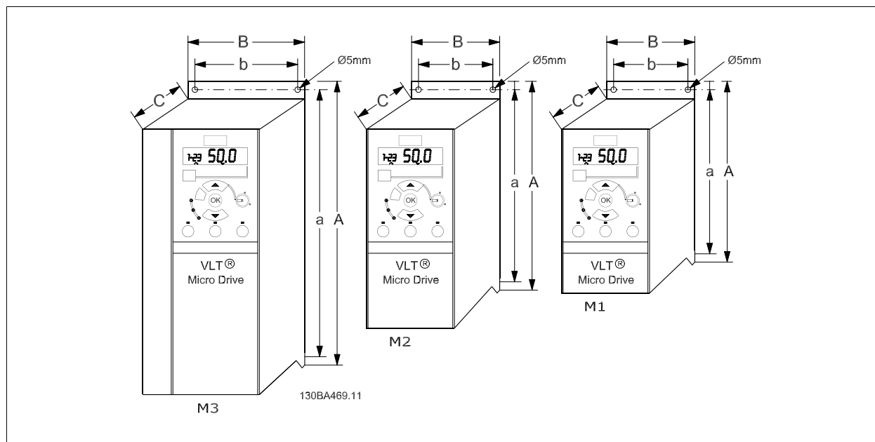
2.3: Mechanical dimensions
