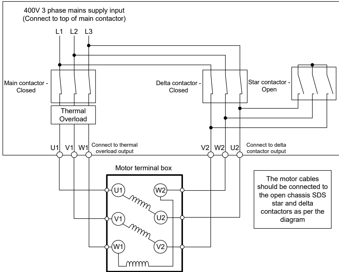
Motor terminals connected in delta
