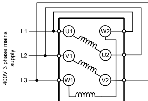
Motor terminals connected in delta
