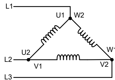
Delta winding connection
