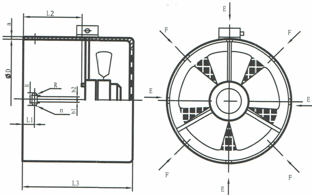
3PH and 1PH Forcevent Dimensions
