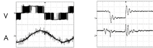
Switching pulse
